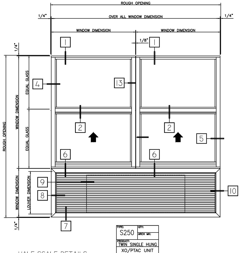
HALF SCALE DETAILS
