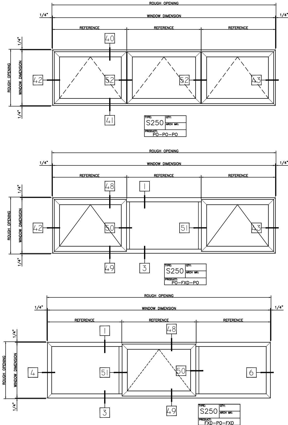
HALF SCALE DETAILS
