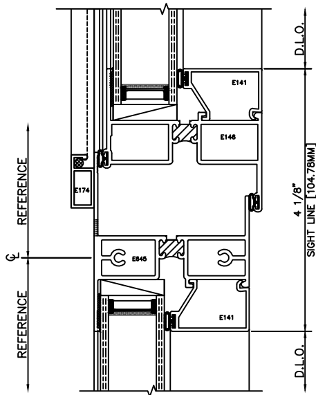
30 MTG RAIL PROJECT IN/FIXED
