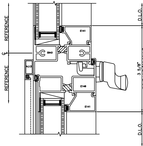
32 MTG RAIL FXD/PROJECT IN
