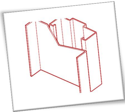
Subjamb Flush Mounted to Door Frame
