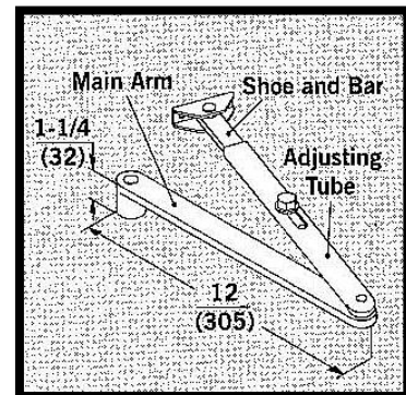
Standard Arm Features Parallel arm, backcheck
